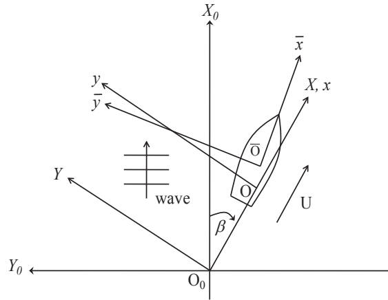
Figure 1. NSM Problem definition
