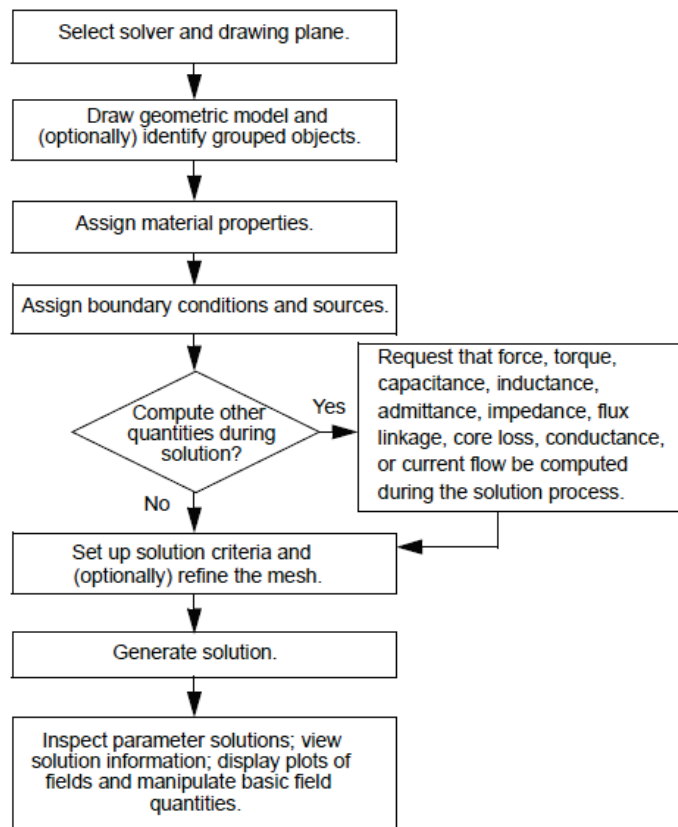
Figure 2. Flowchart of Ansoft Maxwell simulation procedure [12]
