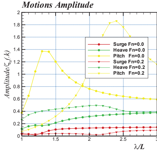
Figure 4. Motion amplitude for F_n=0.0 and F_n=0.2 [4]
